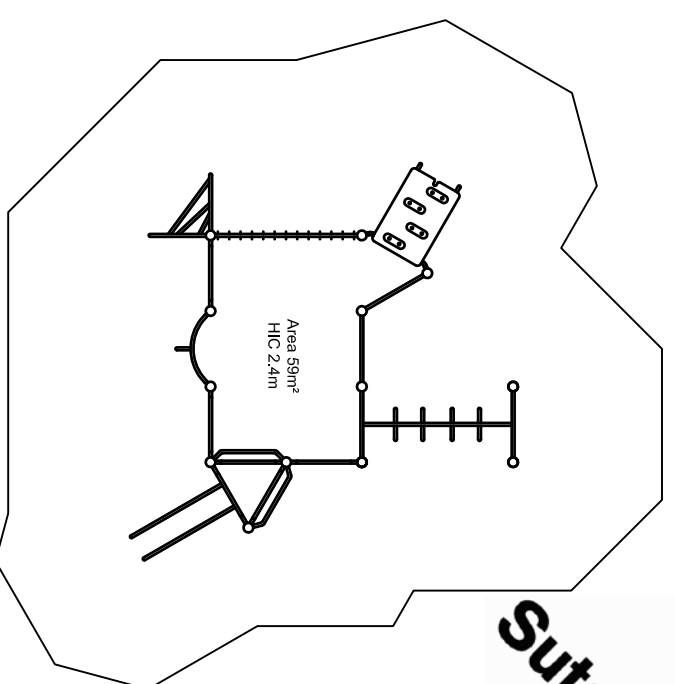
PLAN SCALE 1:100
