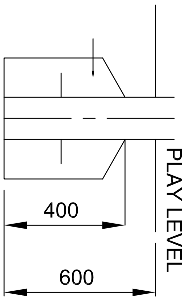
FOUNDATION DETAIL TO EN1176
