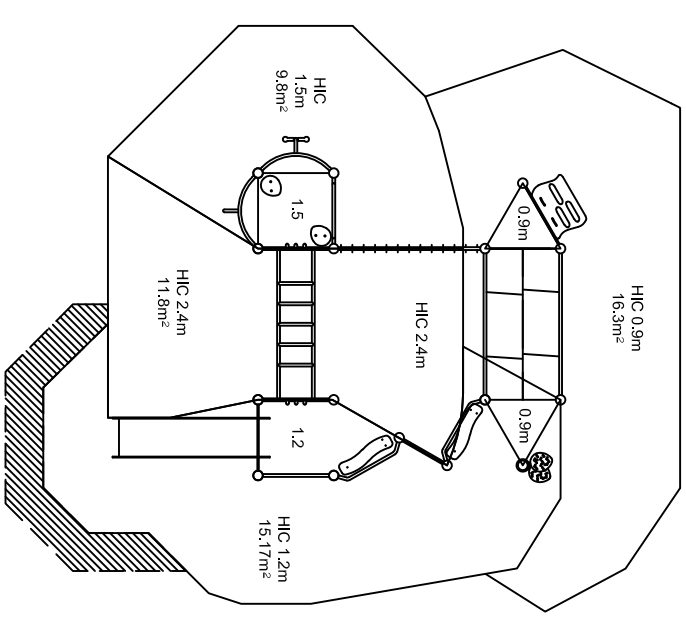
PLAN SCALE 1:100
