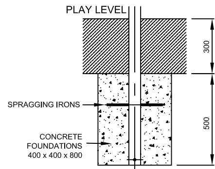
DETAILS OF FOUNDATION HOLE TYPE B SCALE 1:20
