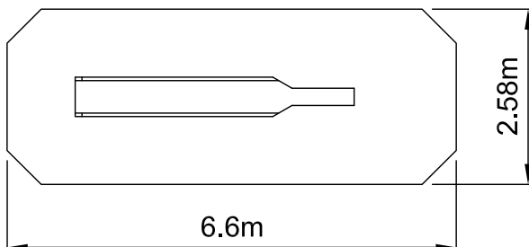
11' EMBANKMENT SLIDE TSL110
