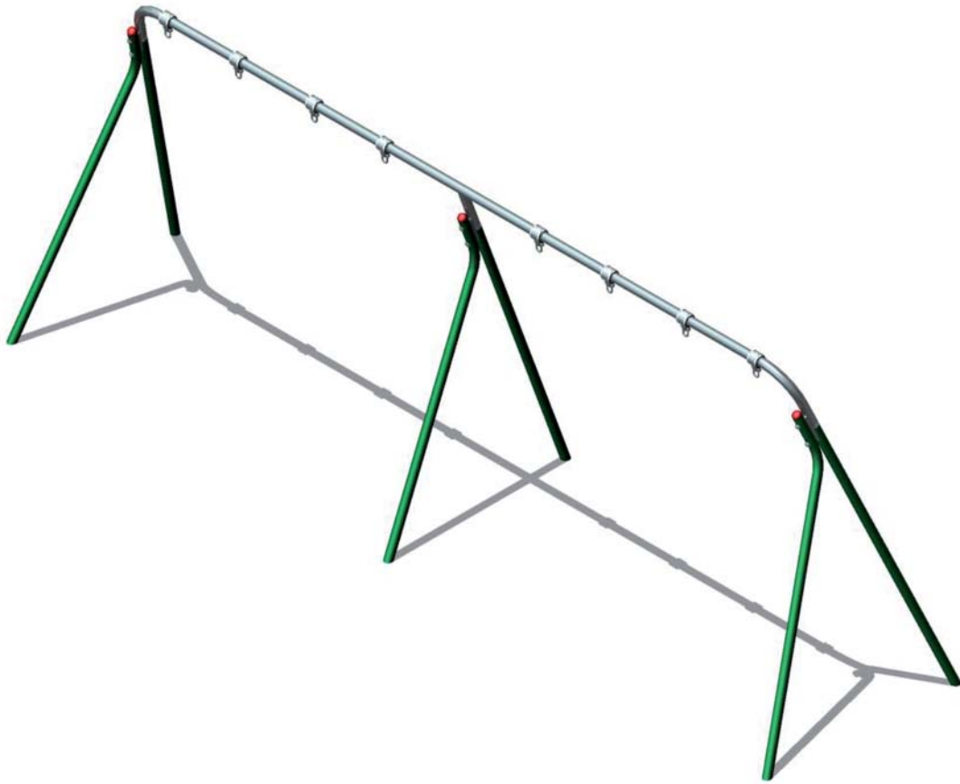
Details for fixing Bent and Straight Legs to the Top Bar
