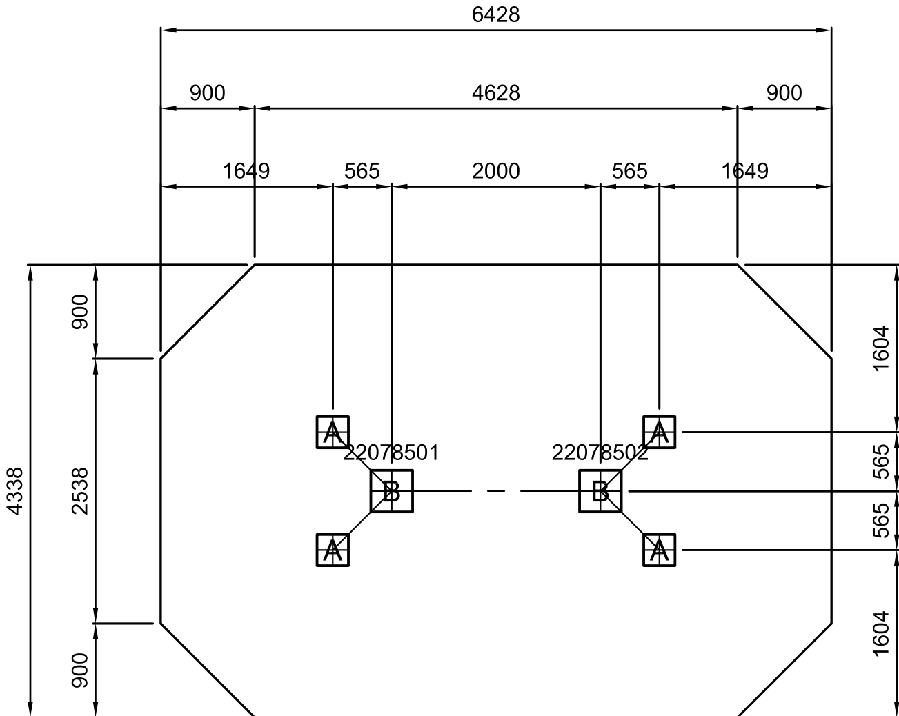
PLAN SCALE 1:100
