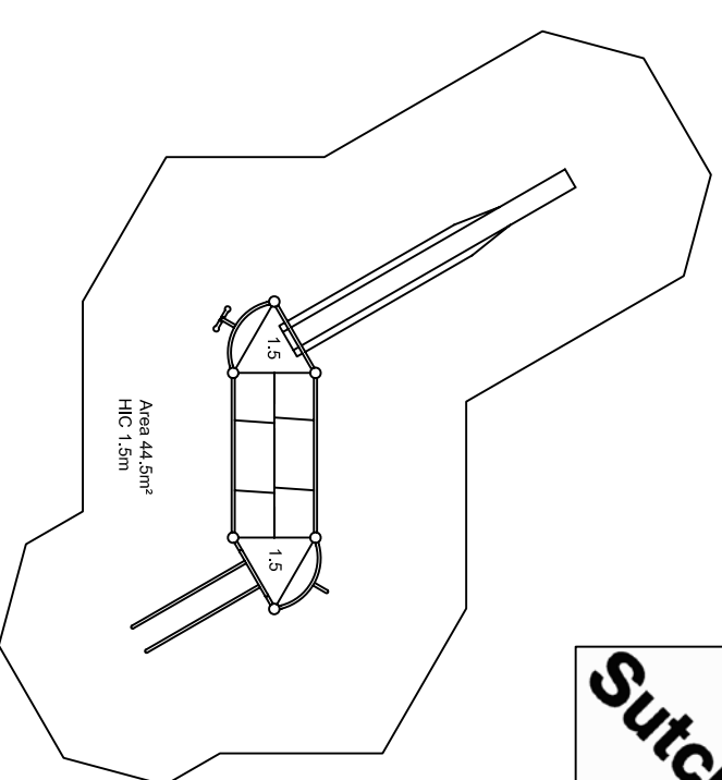
PLAN SCALE 1:100
