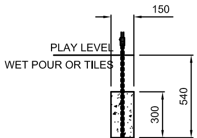
FOUNDATION DETAIL HOLE B FOR NET CHAIN SCALE 1:25
