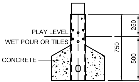
FOUNDATION DETAIL HOLE A TO EN1176 SCALE 1:25
