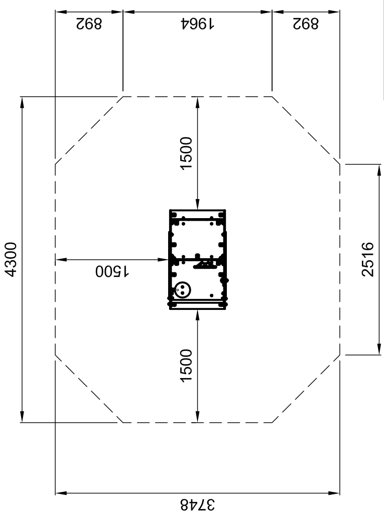
PLAN SCALE 1:50
