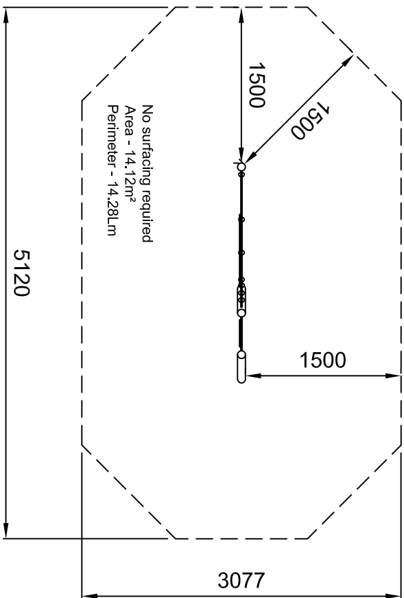
PLAN SCALE 1:50
