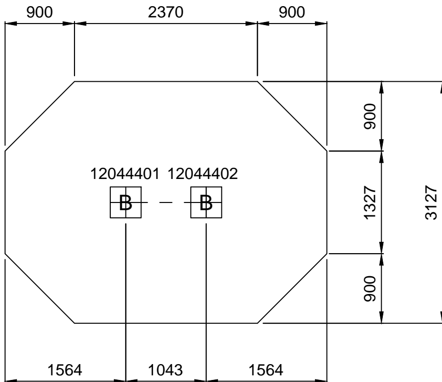
PLAN SCALE 1:100
