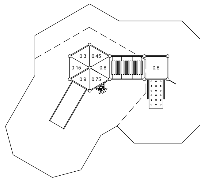
PLAN SCALE 1:100
