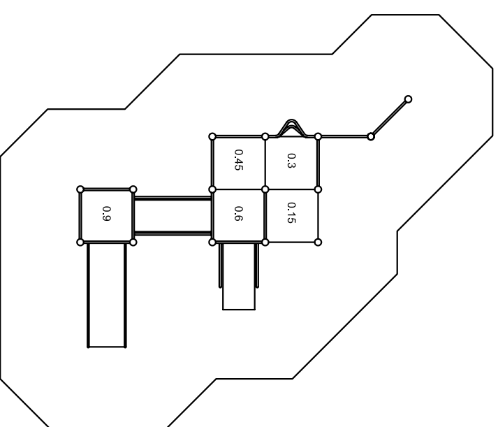
PLAN SCALE 1:100
